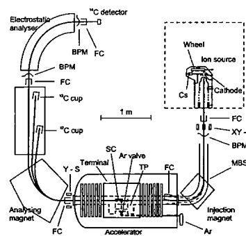
Compact AMS, TV = 0.5 MV 6 m x 5 m = 30 m 2 POZNAN
